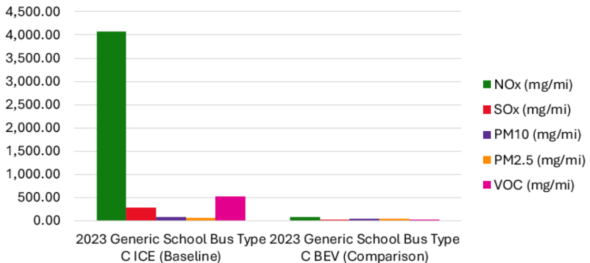
Well-to-Wheel Other Emissions
